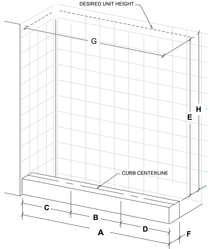
Door w/ 2 Inline Panels
