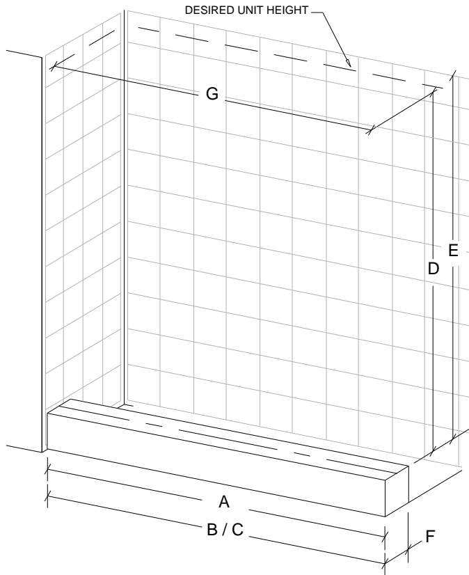
Door w/ Inline Panel
