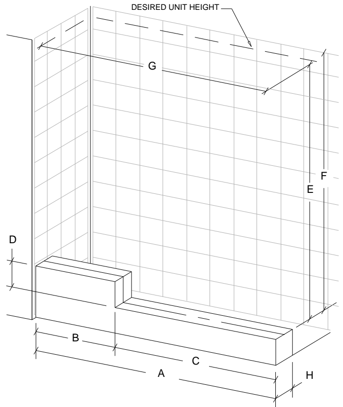
Door w/ Inline Panel ( inline panel on a buttness )
