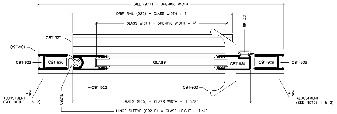
horizontal cross section
